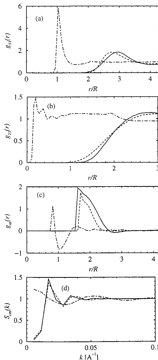
FIG. 15. The effect of rim charges at a concentration of 3% clay by weight: (a) g_{11}(r) , (b) g_{23}(r) , (c) g_{00}(r) , and (d) S_{CM}(k) . Shown are, for model A, the \lambda_D = 3 nm state A9 (solid curves) and for model B, the \lambda_D = 0.96 nm (dashed-dotted) and \lambda_D = 3 nm (dotted curves) states B3, respectively, B4.
